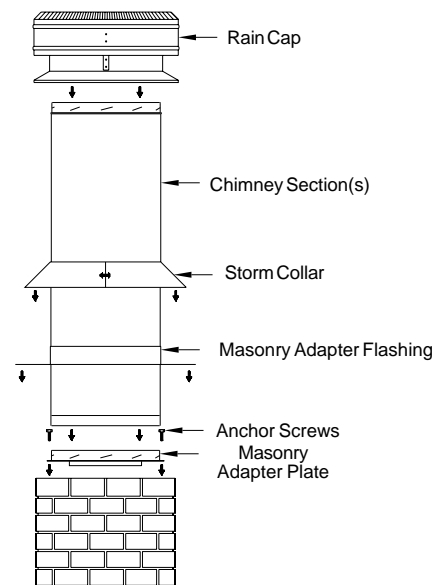
FIGURE 30 Masonry Adapter Installation
