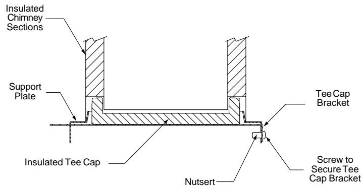
FIGURE 15 - Securing of Insulated Tee Cap
